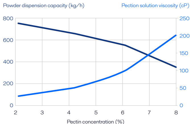
Alfa Laval Hybrid Powder Mixer: The effect of pectin concentration on dispersion capacity and pectin solution viscosity.
