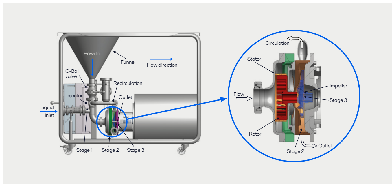
Figure 4. Details of the turbine used in the Alfa Laval Hybrid Powder Mixer.
